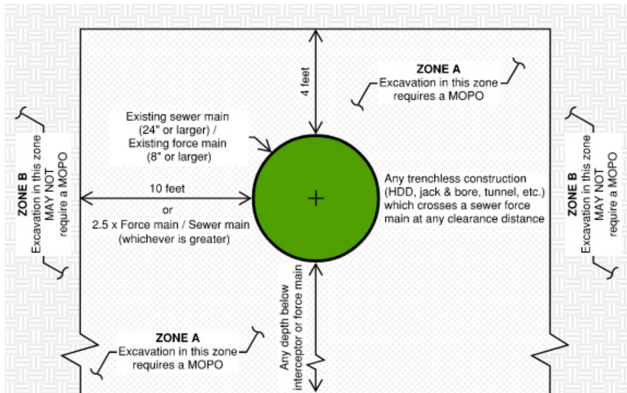
Figure 5. MOPO Requirements for Excavation Near a Sewer Force Main or Sewer Main
