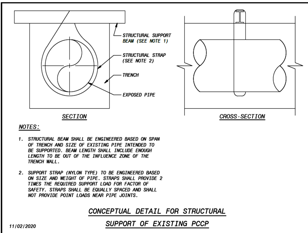
Figure 9. Conceptual Detail for Structural Support of PCCP.
