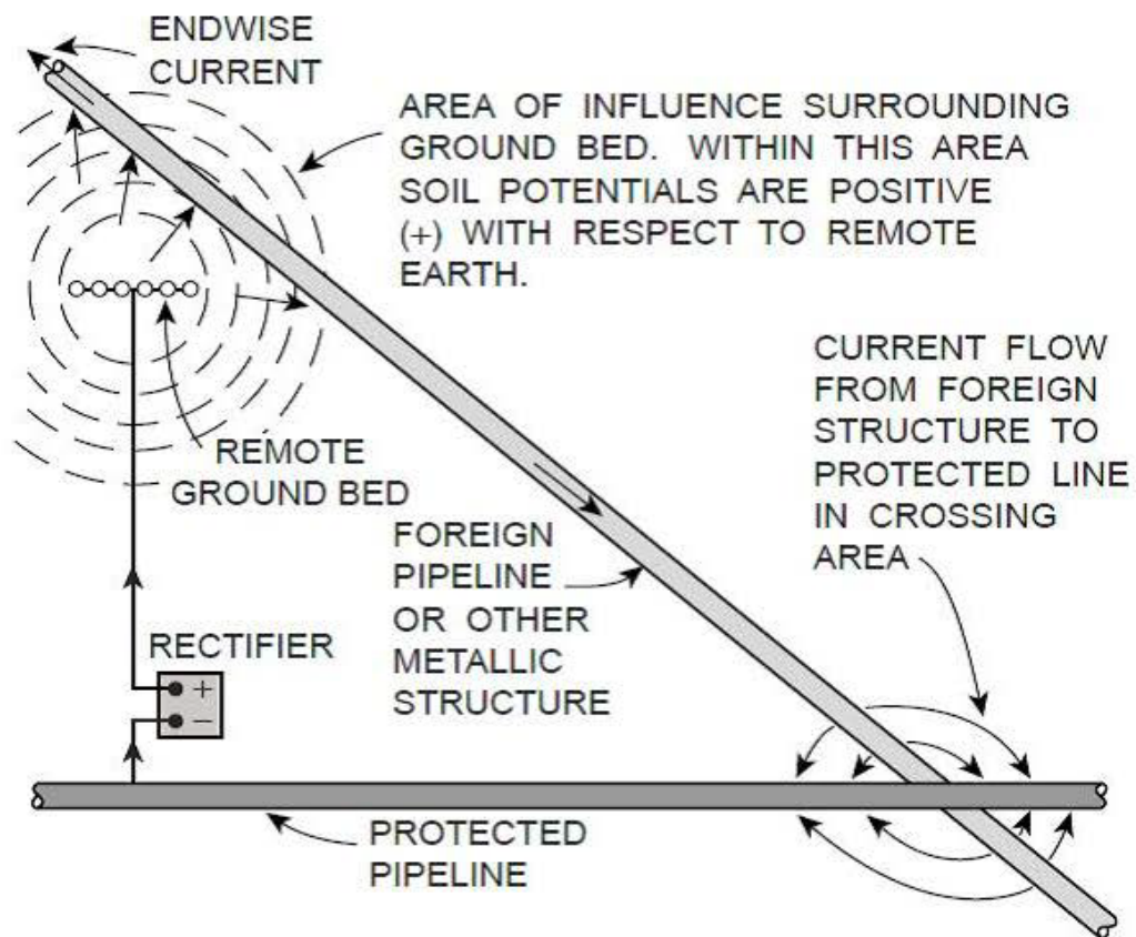
Figure 1 Stray Current Interference from Peabody's Control of Pipeline Corrosion
