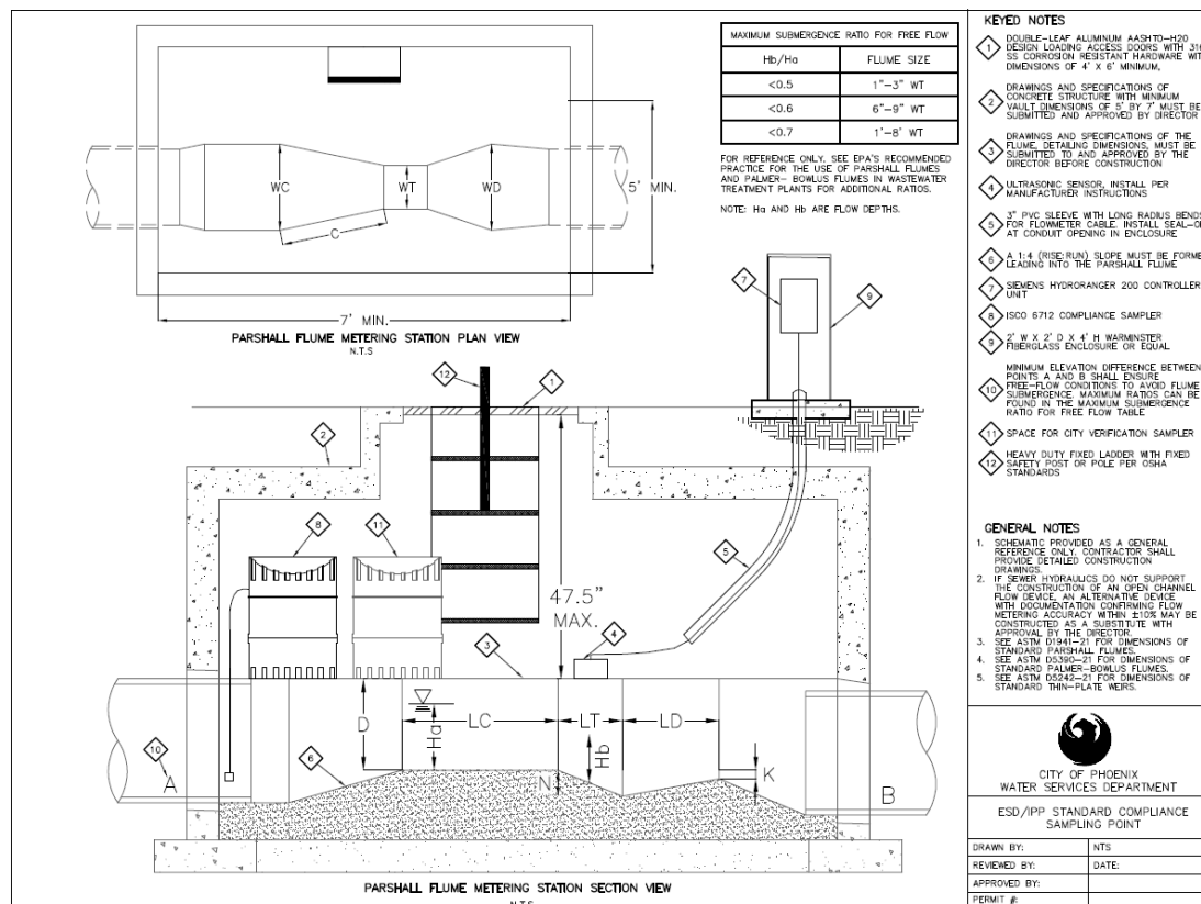
Figure 11. Detail for ESD/IPP Standard Compliance Sampling Point
