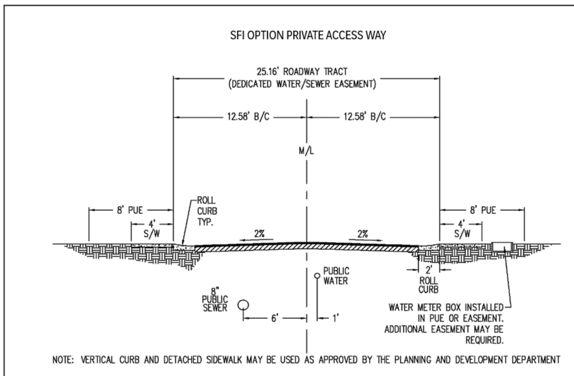
Figure 2. SFI Accessway.
