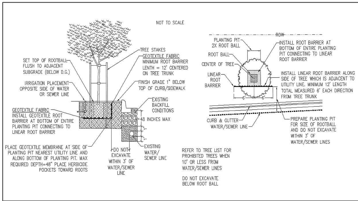
Figure 3. Plant Root Barrier Detail.
