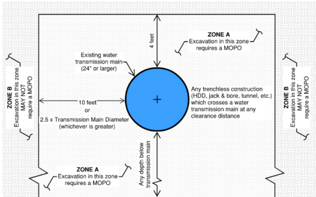
Figure 4. MOPO Requirements for Excavation Near a Water Transmission Main.
