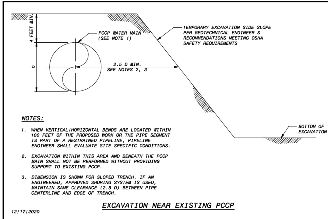
Figure 8. Excavations Near PCCP.
