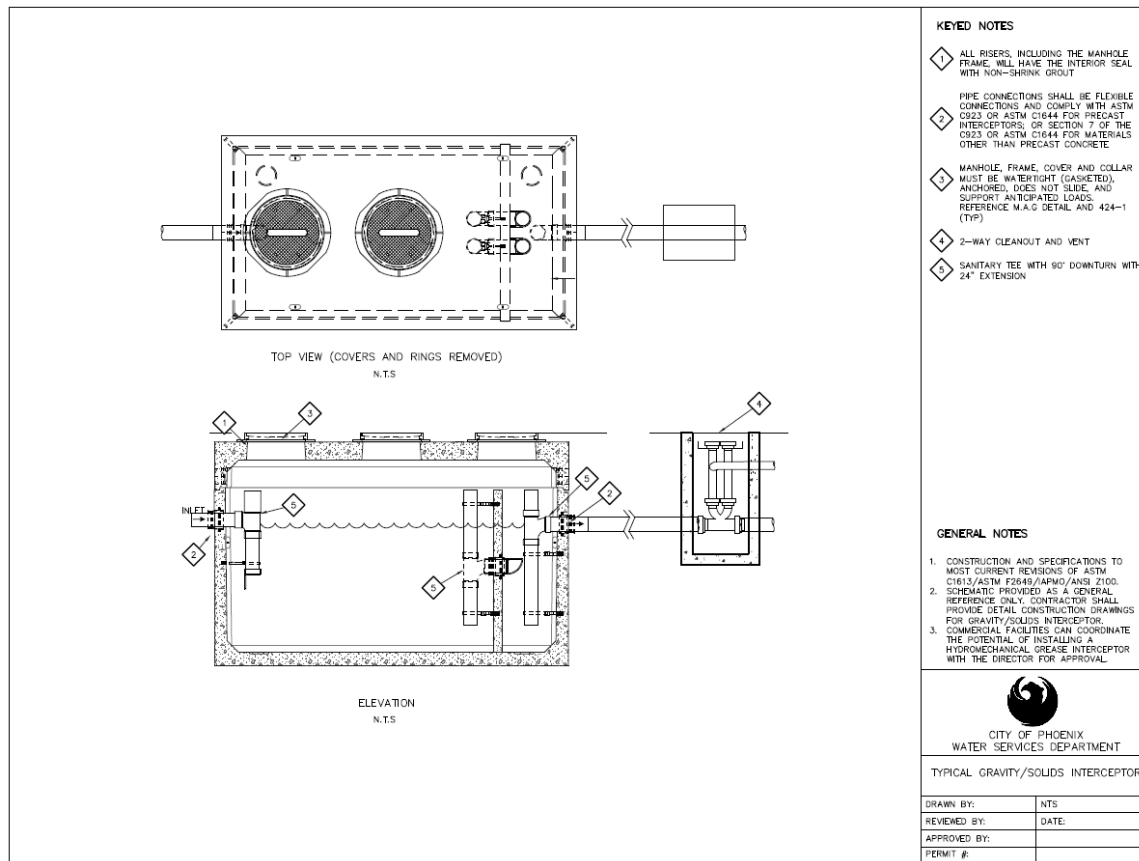
Figure 12. Typical Gravity/Solids Interceptor
