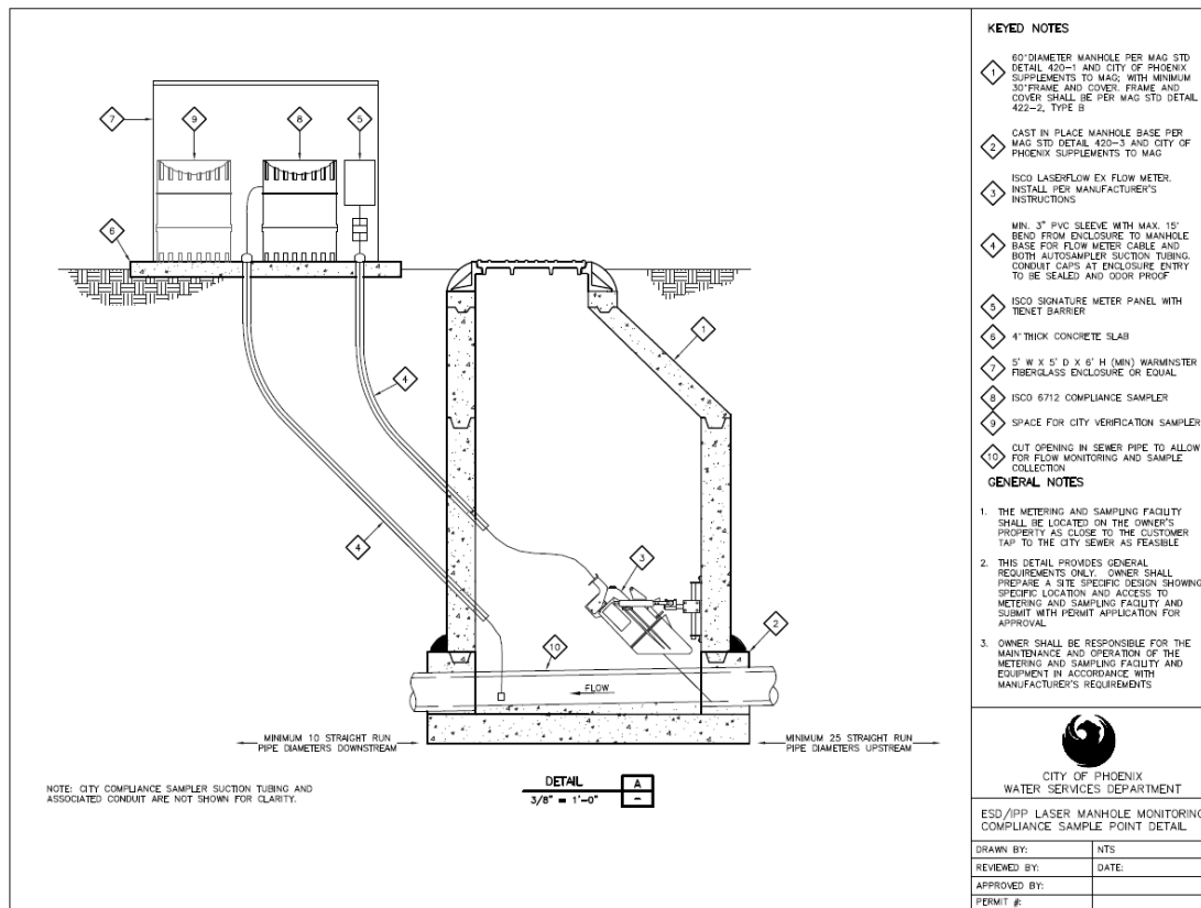
Figure 10. Detail for ESD/IPP Laser Manhole Monitoring Compliance Sample Point Detail
