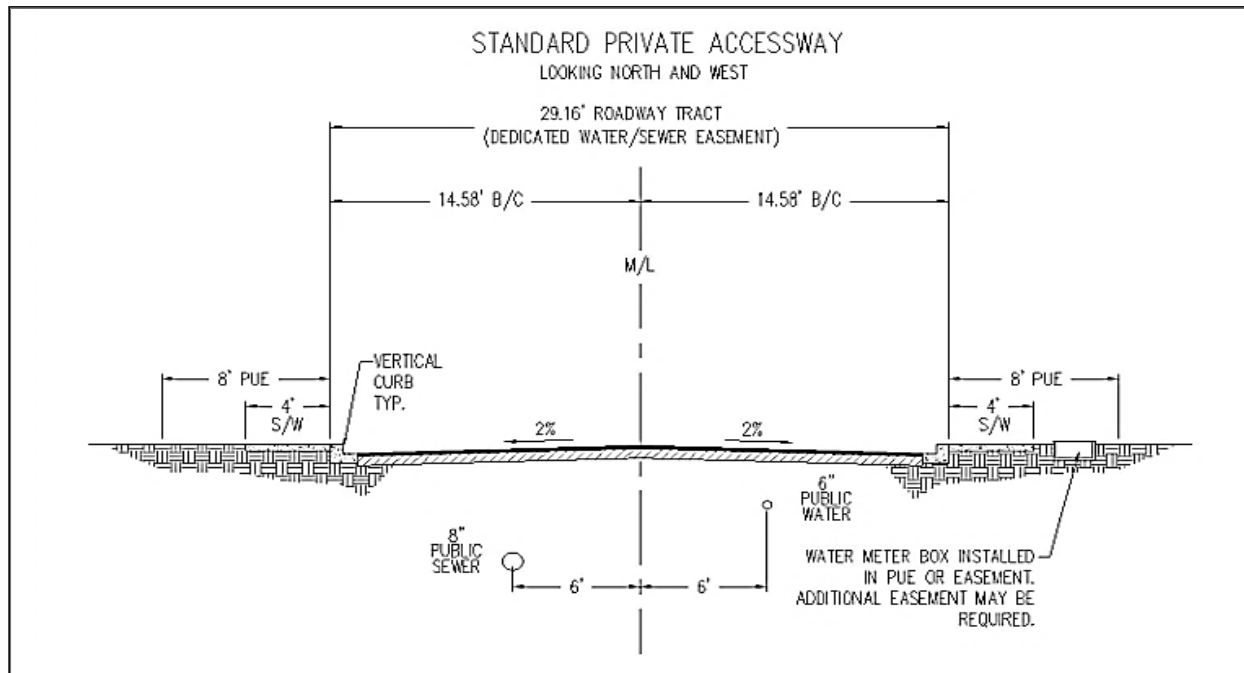
Figure 1. Standard Private Accessway.
