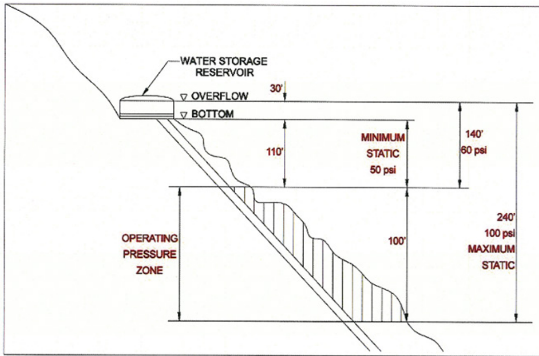
Figure 6. Typical Major Water Pressure Zone Configuration (rounded to the nearest 10 psi).
