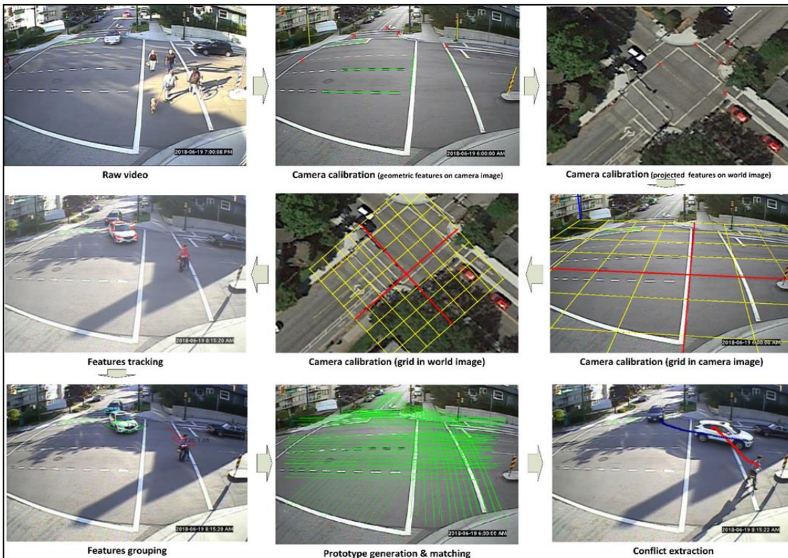
Figure 6: A Diagram of the Process of Traffic Conflict Analysis (Y. Guo et al., 2020)
