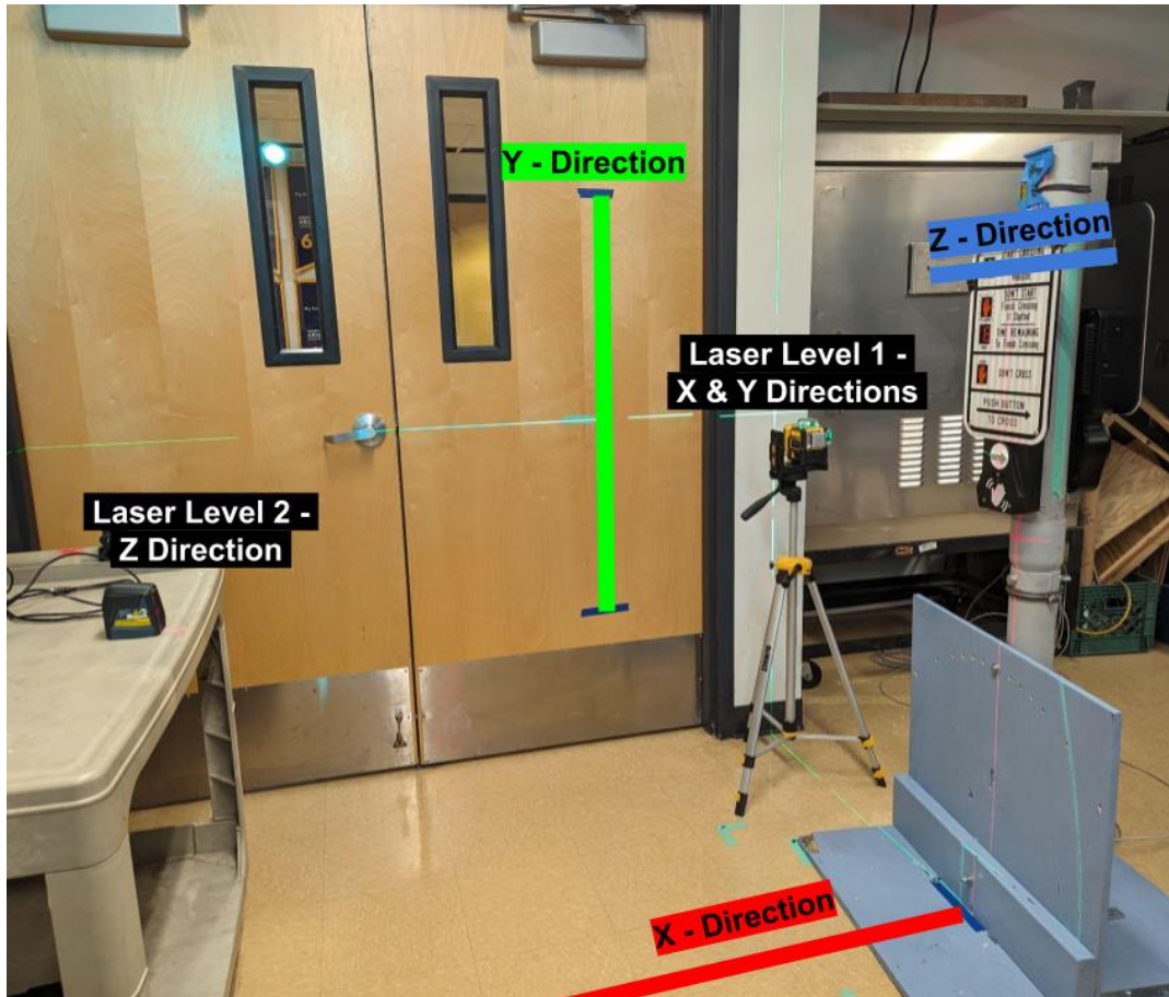
Figure 18: Testing Apparatus
