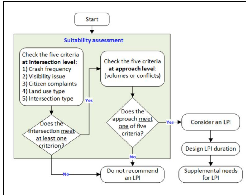
Figure 3: FDOT’s Preliminary Suitability Assessment and Design Recommendation Flowchart (Lin et al., 2017)
