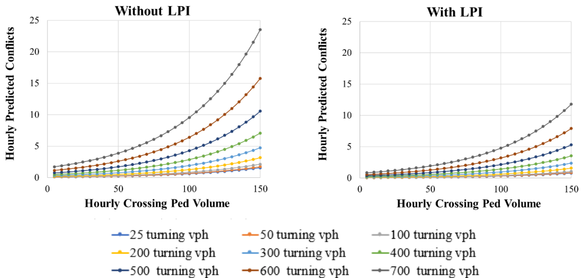
Figure 33: Predicted hourly conflict frequency with and without LPI treatment.
