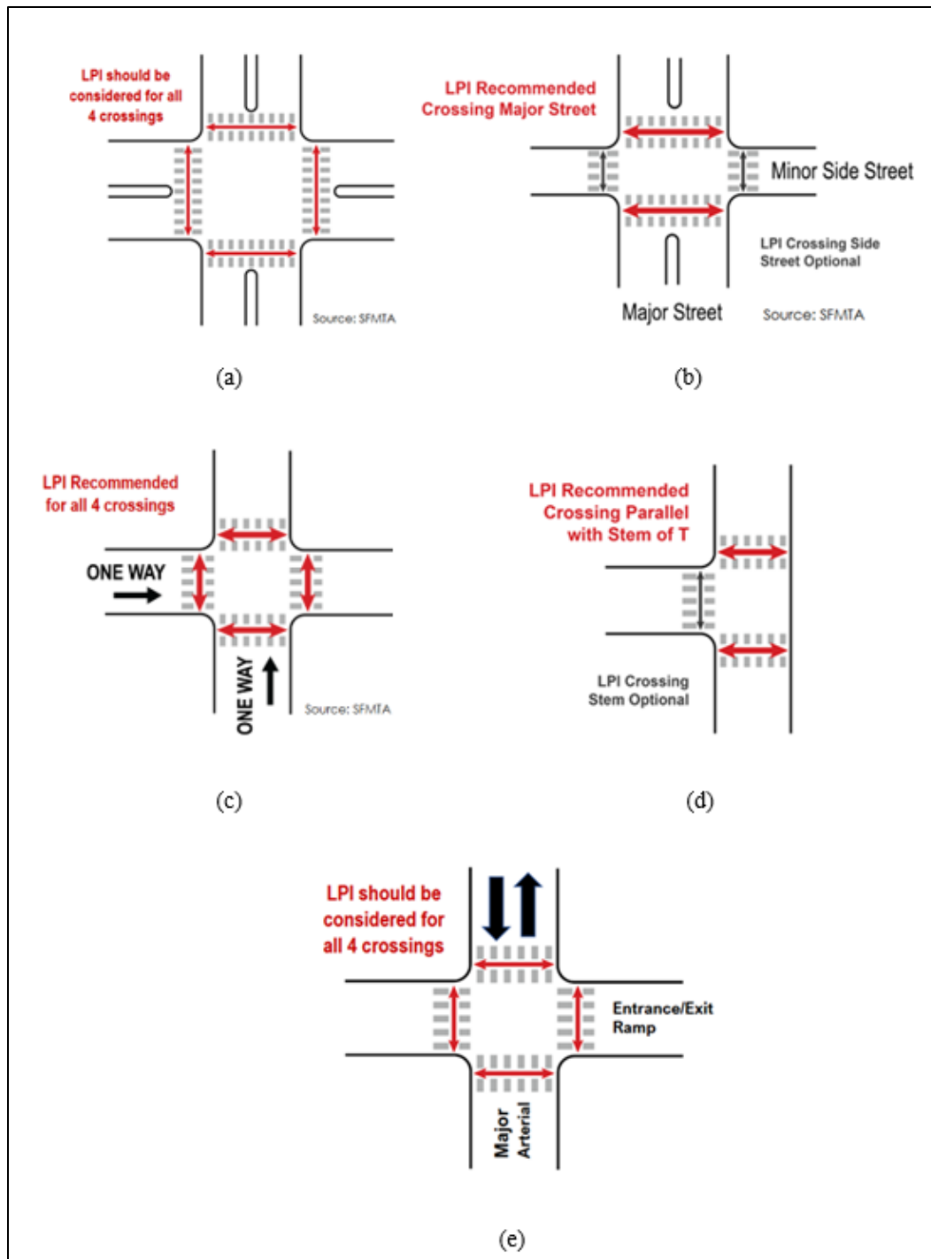
Figure 4: LPIs at Typical Intersections
