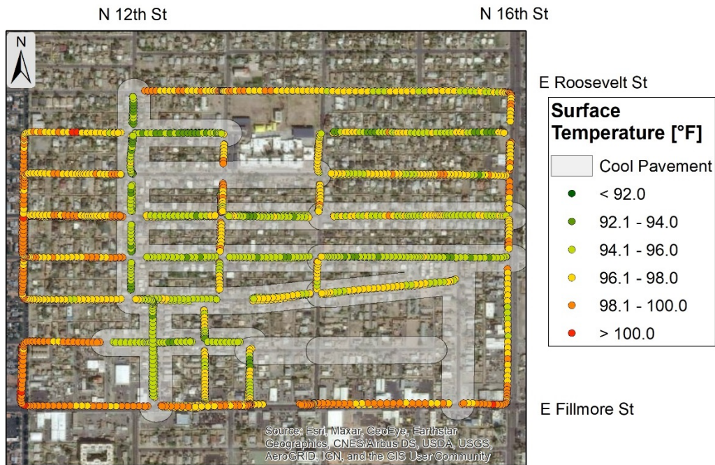
Figure A1. Map of measured and time-detrended surface temperature for 4:50 AM on August 18, 2020, in the Garfield neighborhood in district 8.
