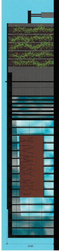
② PHASE 2 CHURCH EAST 3/32" = 1'-0"
